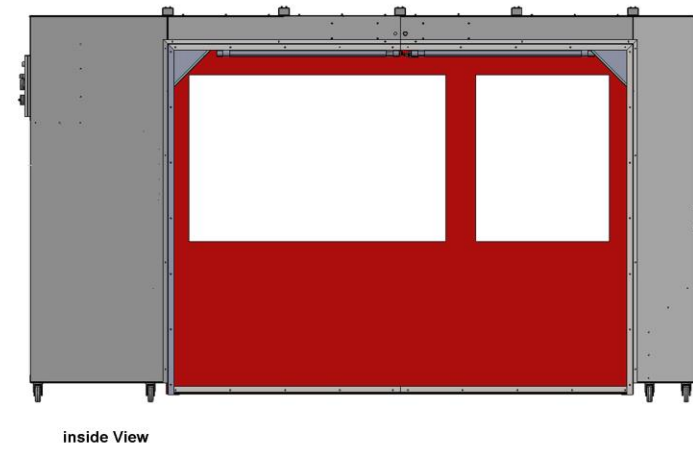
Spray Booth Dimensions Are approx
